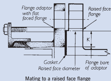
Mating to a raised face flange
