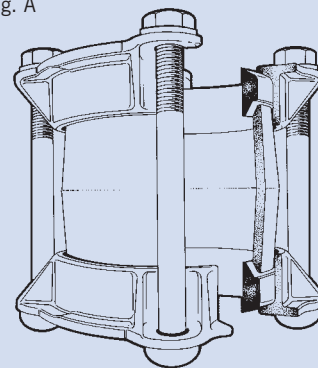
Cutaway illustration of Helden straight coupling.
