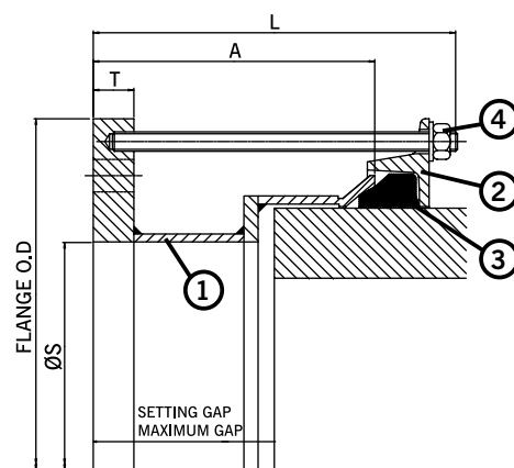
Flange Adaptor Type 3
