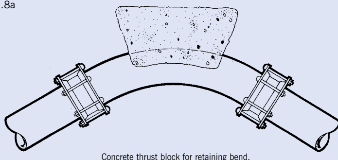
Concrete thrust block for retaining bend.
