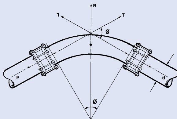
Longitudinal pressure forces acting at a bend.
